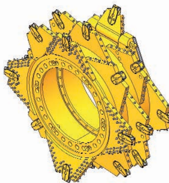
Four tooth holders in one row of teeth
