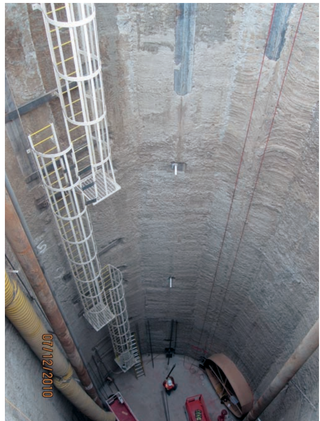
CSM-wall for start shaft microtunneling (USA)
